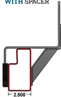
PALLET STOP WITH SPACER
